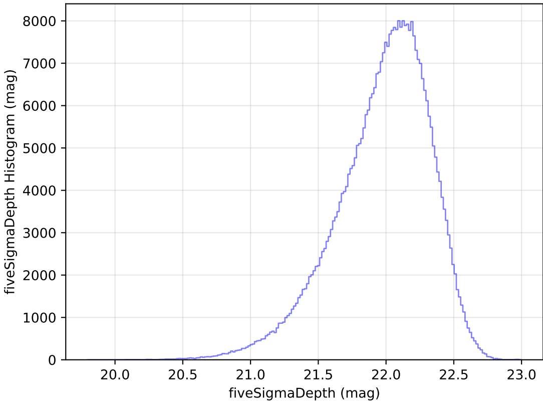
too_elab_r64_d3_ugrizy_v3.4_10yrs y: fiveSigmaDepth Histogram
