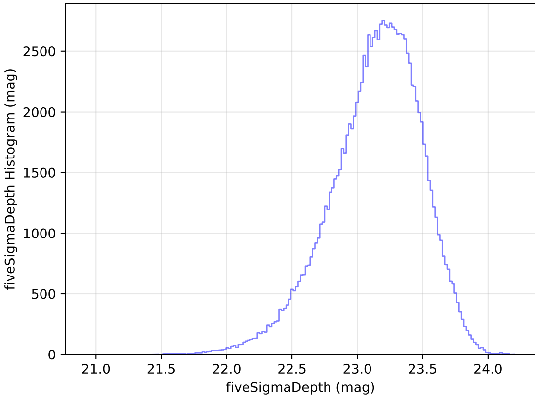
too_elab_r64_d3_ugrizy_v3.4_10yrs u: fiveSigmaDepth Histogram
