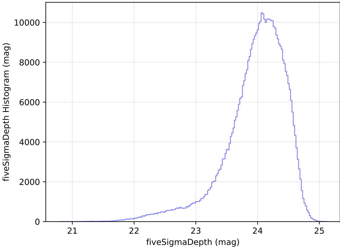
too_elab_r64_d3_ugrizy_v3.4_10yrs r: fiveSigmaDepth Histogram
