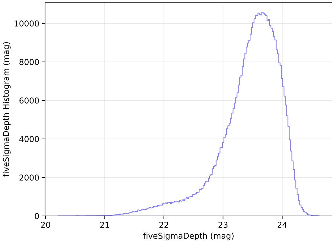
too_elab_r64_d3_ugrizy_v3.4_10yrs i: fiveSigmaDepth Histogram
