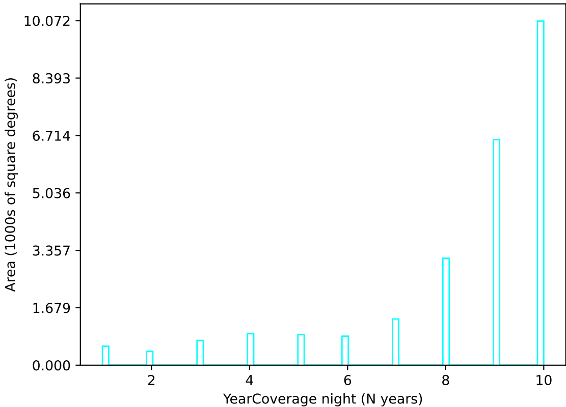
too_elab_r64_d3_uigrzy_v3.4_10yrs u band: YearCoverage night
