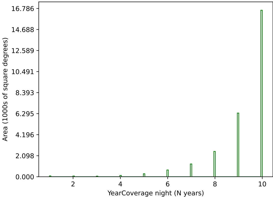
too_elab_r64_d3_ugrizy_v3.4_10yrs g band: YearCoverage night
