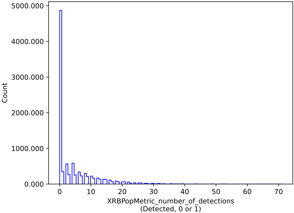
too_elab_r64_d3_ugrizy_v3.4_10yrs : XRBPopMetric_number_of_detections
