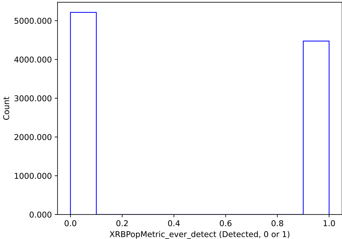
too_elab_r64_d3_ugrizy_v3.4_10yrs : XRBPoMetric_ever_detect
