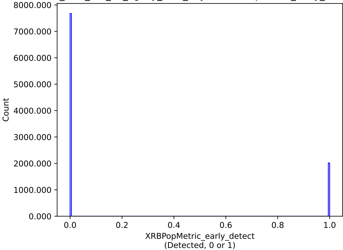
too_elab_r64_d3_ugrizy_v3.4_10yrs : XRBPopMetric_early_detect
