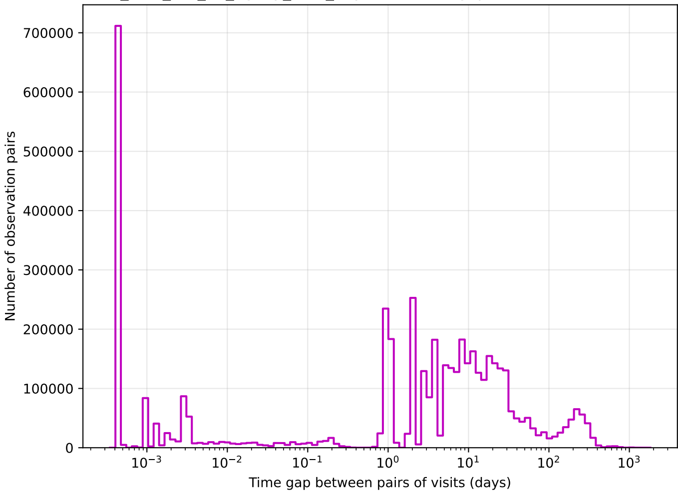
too_elab_r64_d3_ugrizy_v3.4_10yrs z band: Tgaps observationStartMJD
