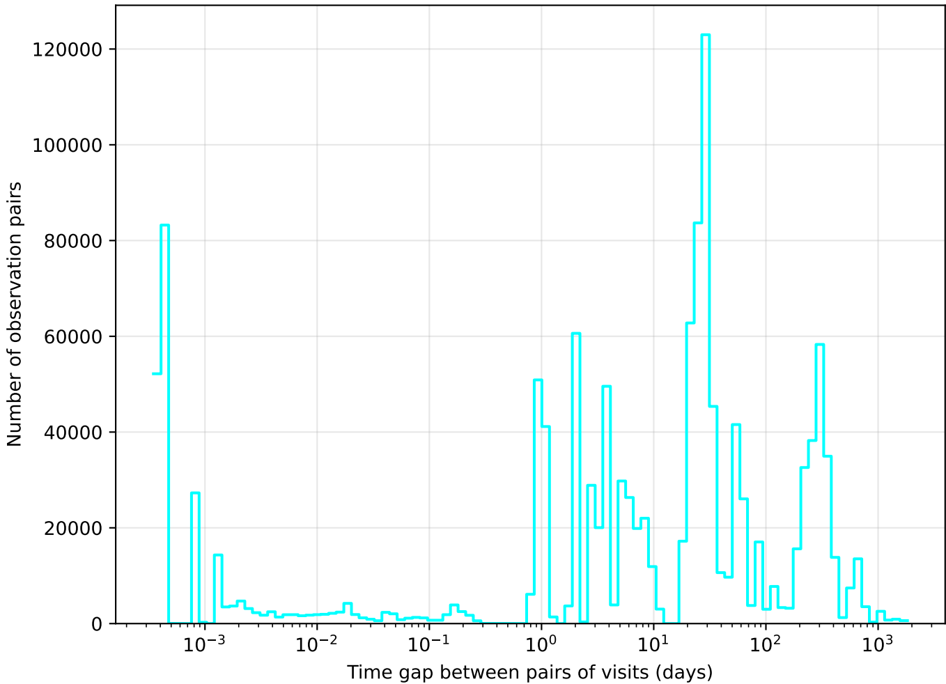
too_elab_r64_d3_ugrizy_v3.4_10yrs u band: Tgaps observationStartMJD
