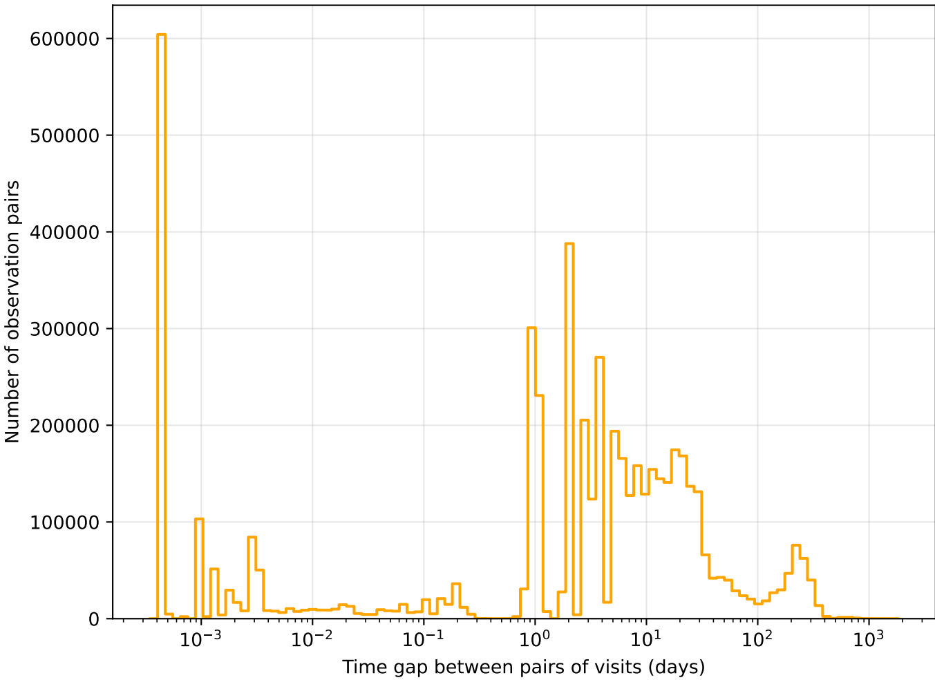
too_elab_r64_d3_ugrizy_v3.4_10yrs r band: Tgaps observationStartMJD
