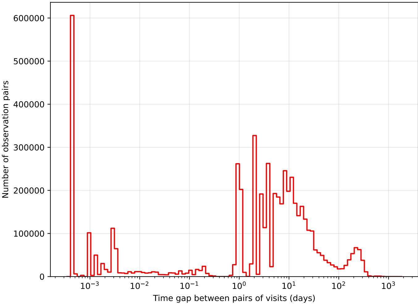
too_elab_r64_d3_ugrizy_v3.4_10yrs i band: Tgaps observationStartMJD
