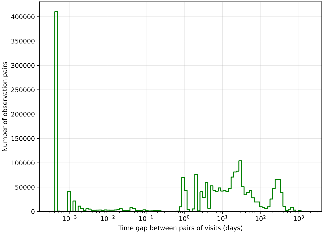
too_elab_r64_d3_ugrizy_v3.4_10yrs g band: Tgaps observationStartMJD
