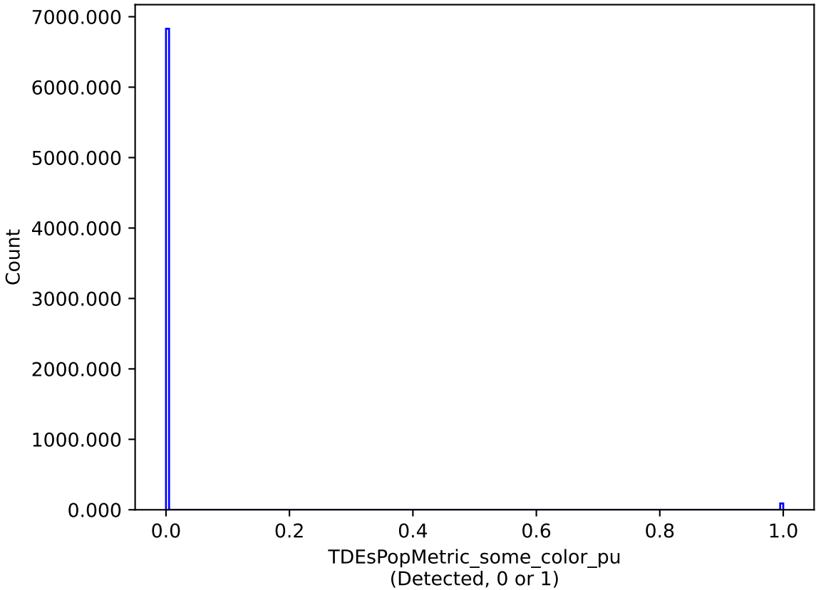
too_elab_r64_d3_ugrizy_v3.4_10yrs : TDEsPopMetric_some_color_pu
