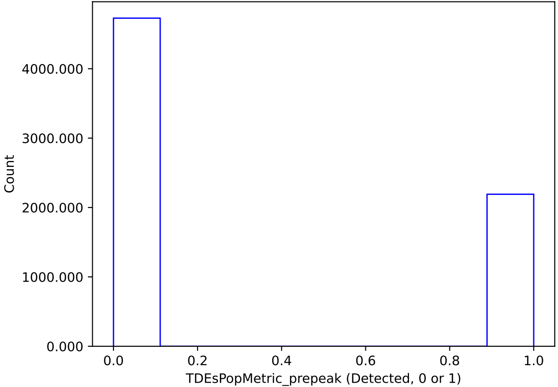
too_elab_r64_d3_ugrizy_v3.4_10yrs : TDEsPopMetric_prepeak
