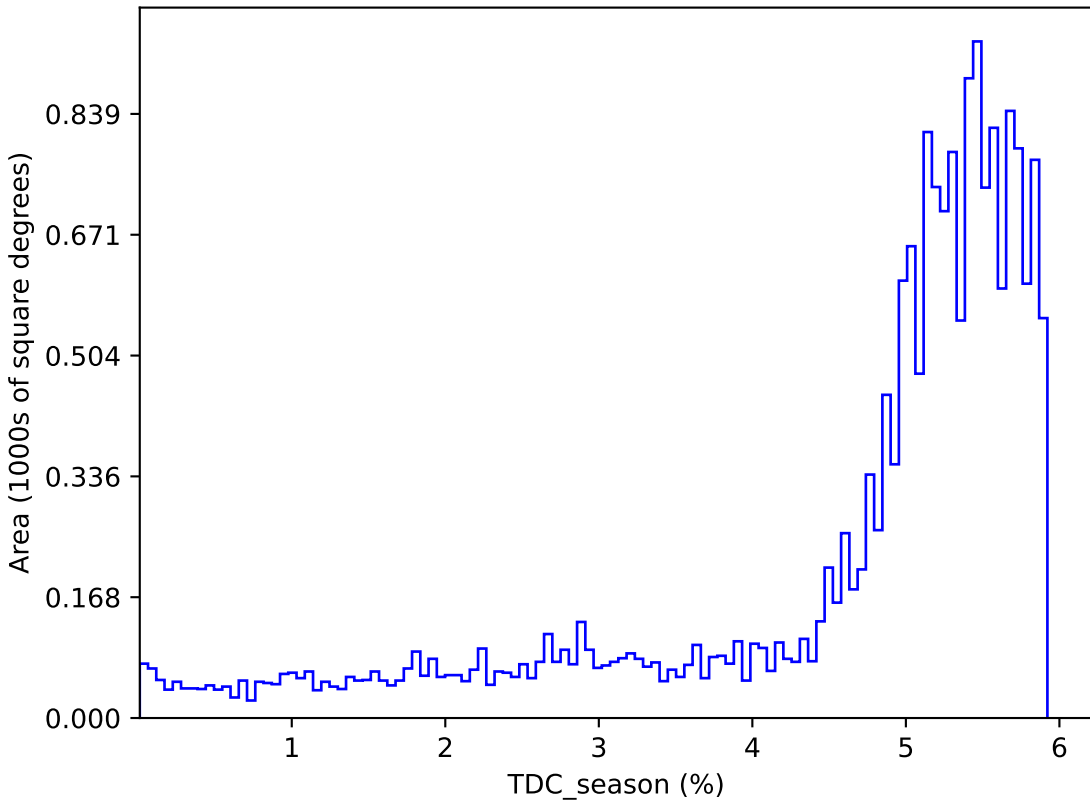
too_elab_r64_d3_ugrizy_v3.4_10yrs : TDC_season
