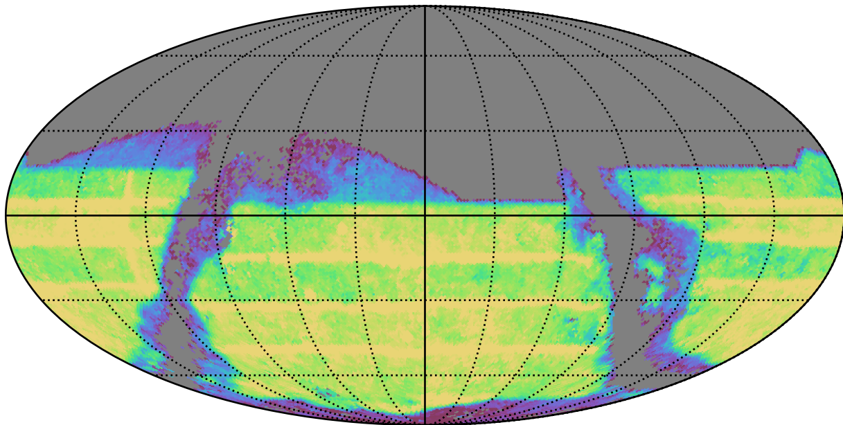
too_elab_r64_d3_ugrizy_v3.4_10yrs : TDC_rate
