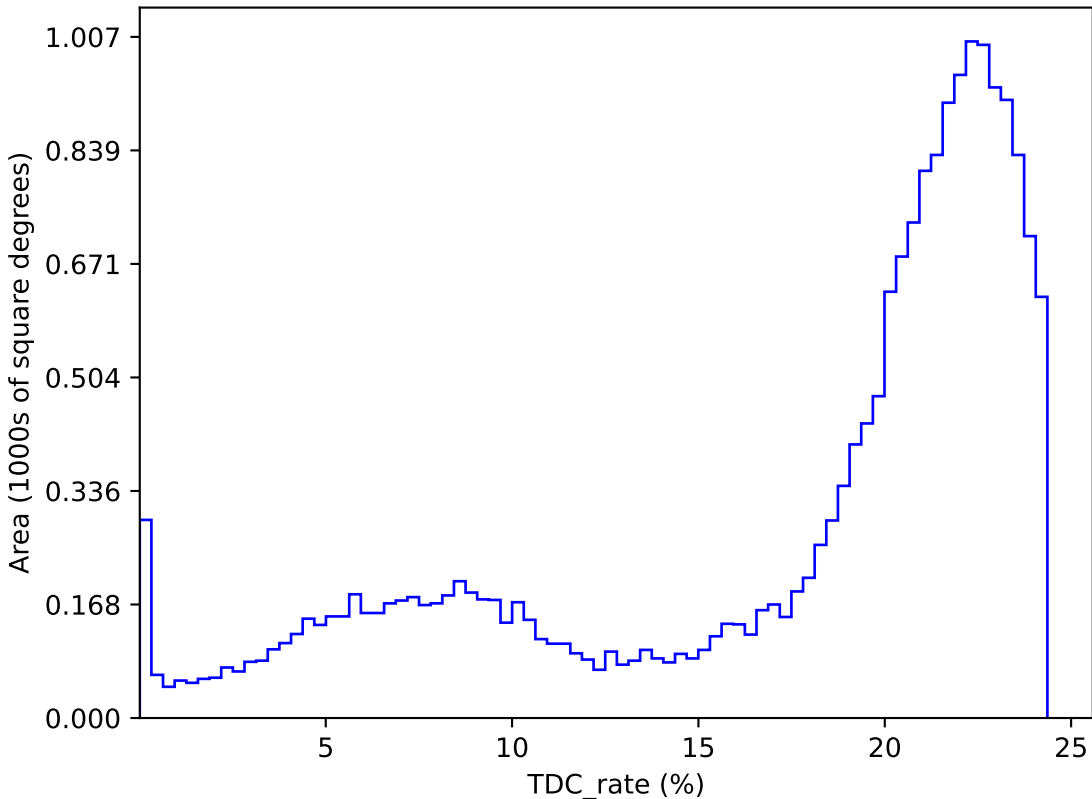
too_elab_r64_d3_ugrizy_v3.4_10yrs : TDC_rate
