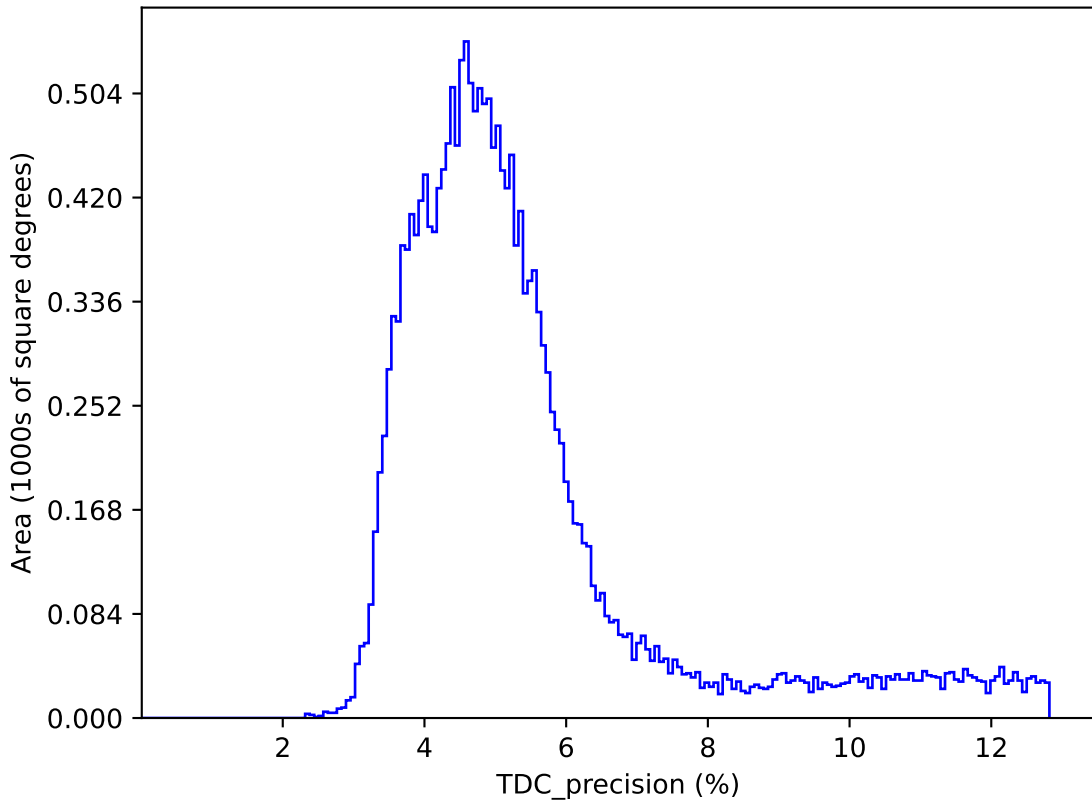
too_elab_r64_d3_ugrizy_v3.4_10yrs : TDC_precision
