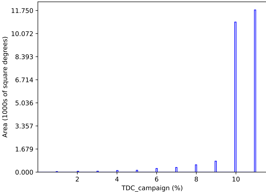
too_elab_r64_d3_ugrizy_v3.4_10yrs : TDC_campaign
