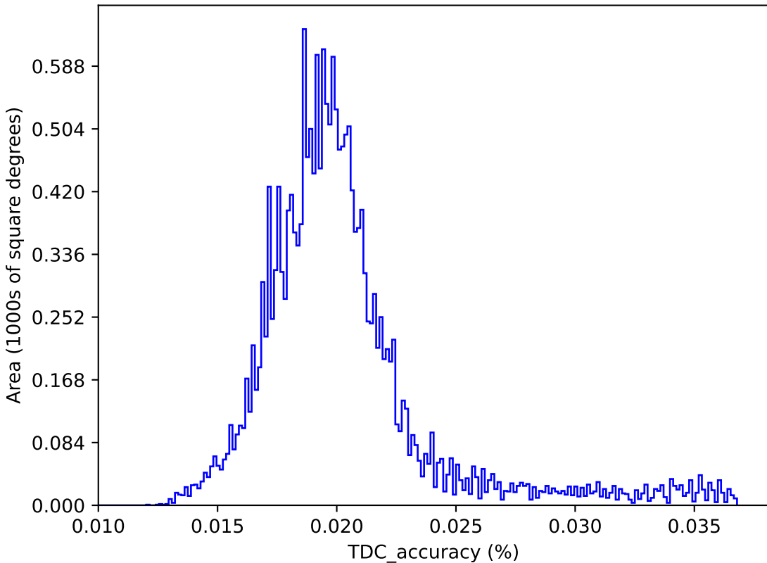
too_elab_r64_d3_ugrizy_v3.4_10yrs : TDC_accuracy
