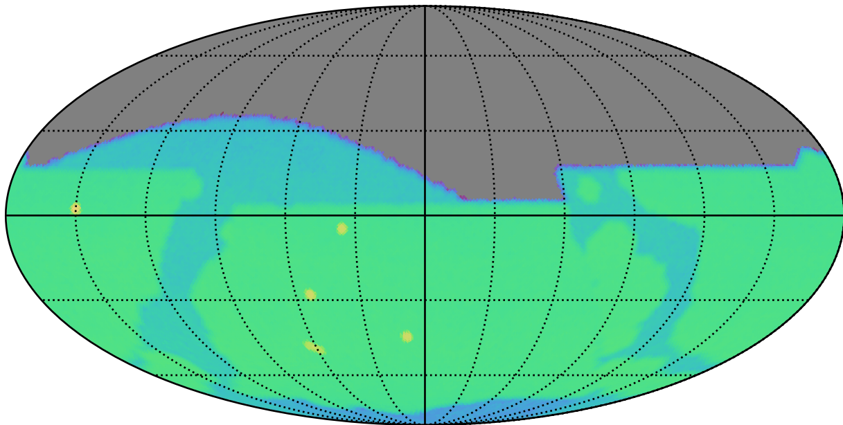
too_elab_r64_d3_ugrizy_v3.4_10yrs r: SurfaceBrightLimit
