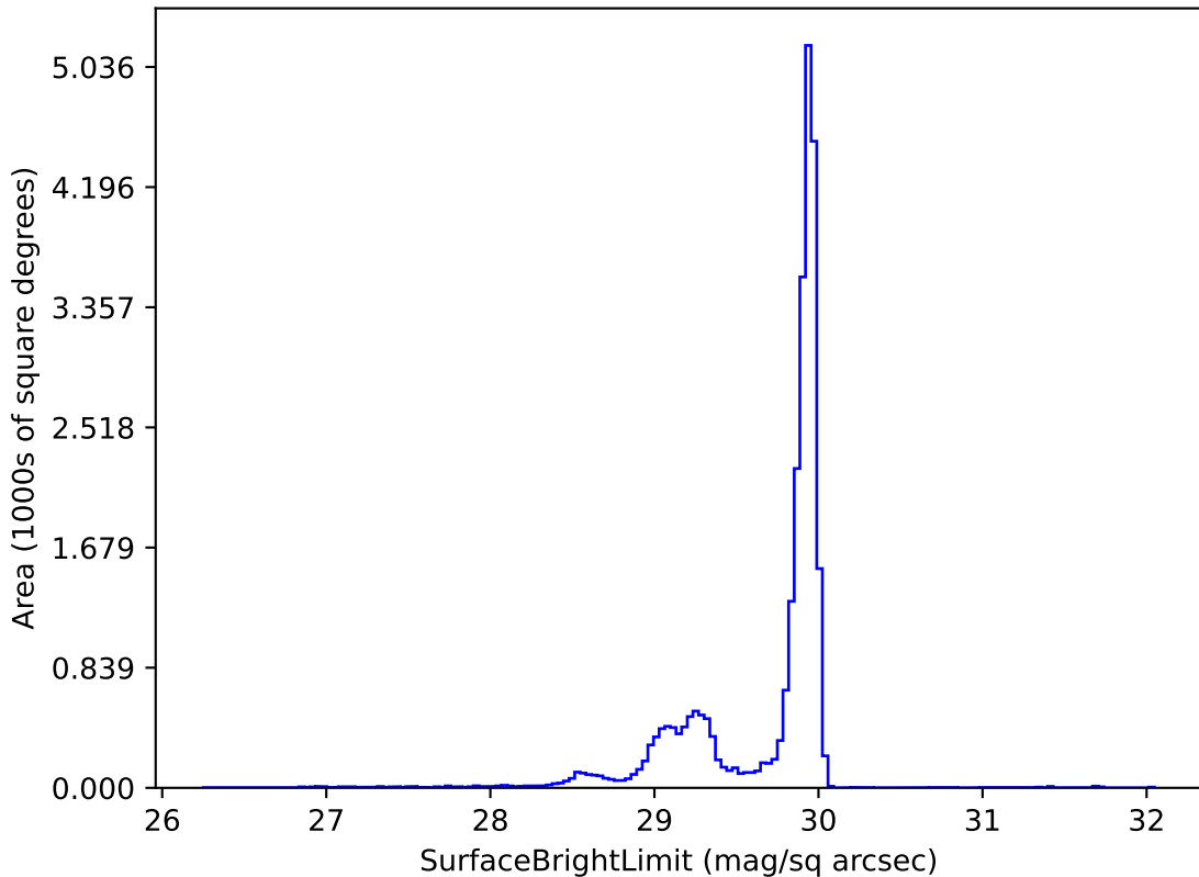
too_elab_r64_d3_ugrizy_v3.4_10yrs i: SurfaceBrightLimit
