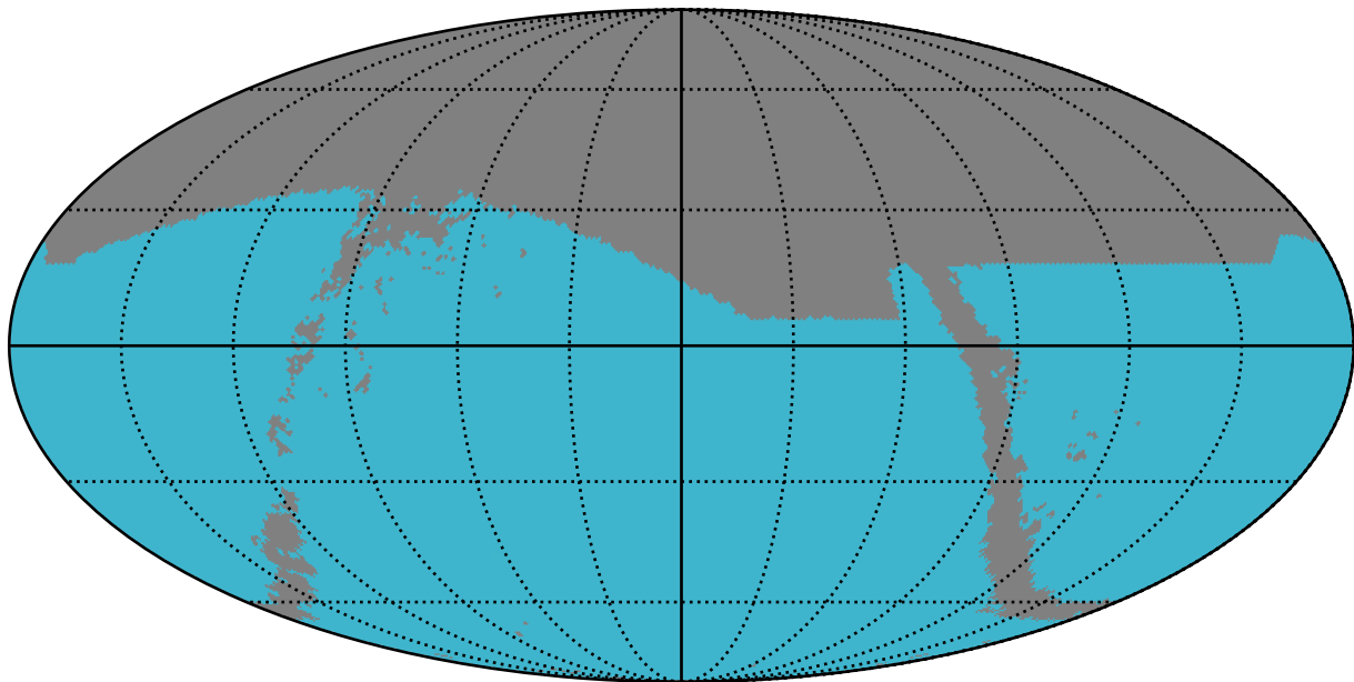
too_elab_r64_d3_ugrizy_v3.4_10yrs : SNSLMetric
