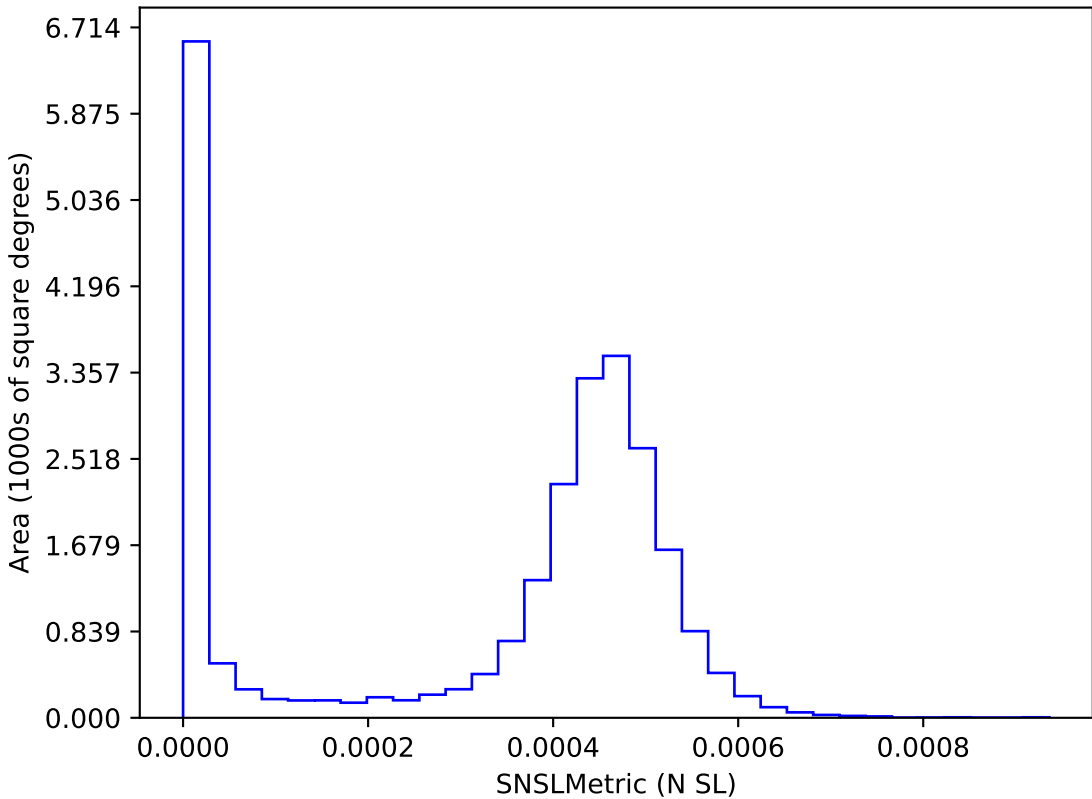
too_elab_r64_d3_ugrizy_v3.4_10yrs : SNSLMetric
