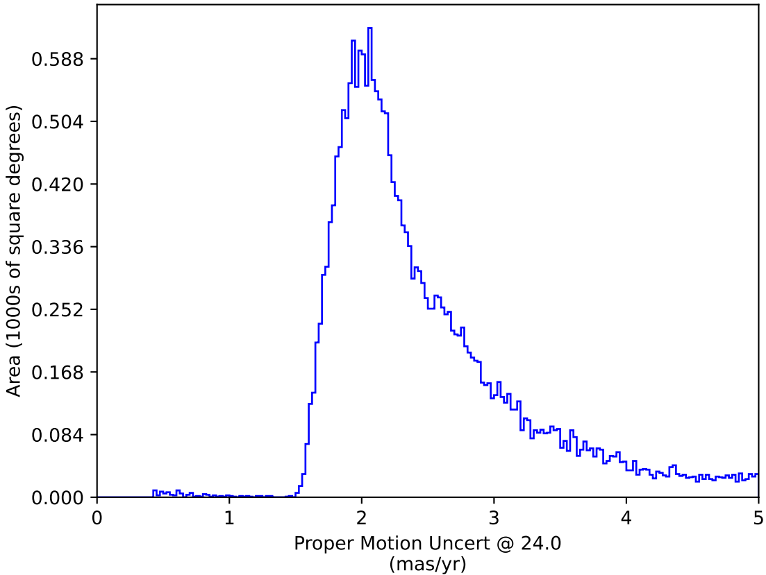
too_elab_r64_d3_ugrizy_v3.4_10yrs : Proper Motion Uncert @ 24.0
