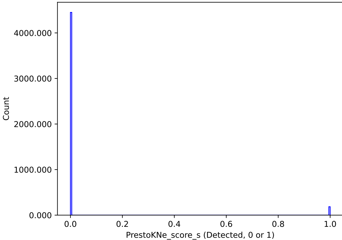
too_elab_r64_d3_ugrizy_v3.4_10yrs : PrestoKNe_score_s
