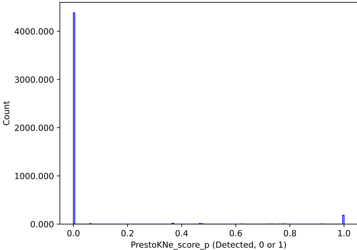
too_elab_r64_d3_ugrizy_v3.4_10yrs : PrestoKNe_score_p
