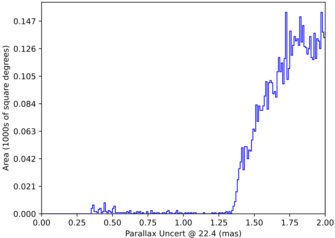
too_elab_r64_d3_ugrizy_v3.4_10yrs : Parallax Uncert @ 22.4
