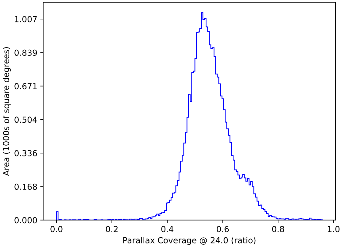
too_elab_r64_d3_ugrizy_v3.4_10yrs : Parallax Coverage @ 24.0
