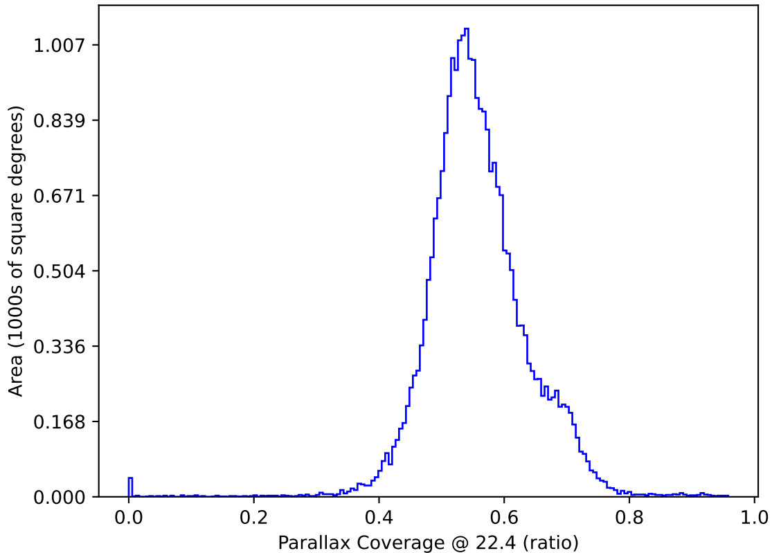
too_elab_r64_d3_ugrizy_v3.4_10yrs : Parallax Coverage @ 22.4
