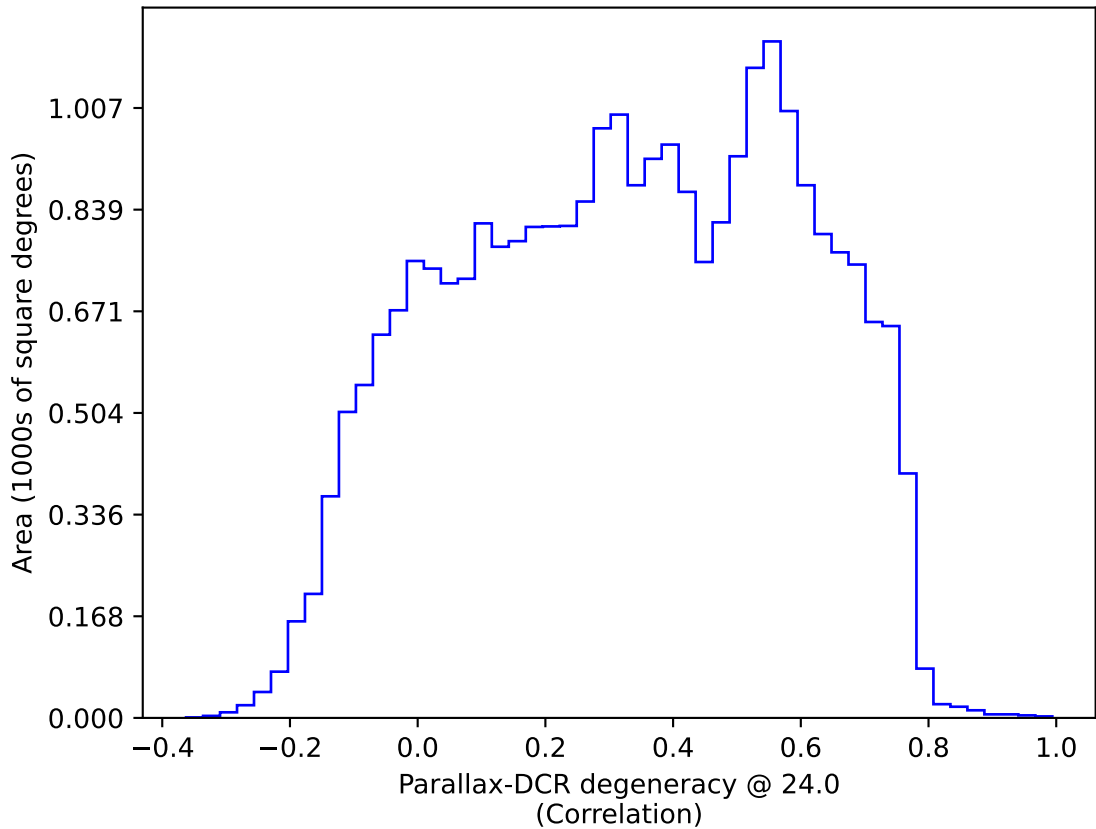
too_elab_r64_d3_ugrizy_v3.4_10yrs : Parallax-DCR degeneracy @ 24.0
