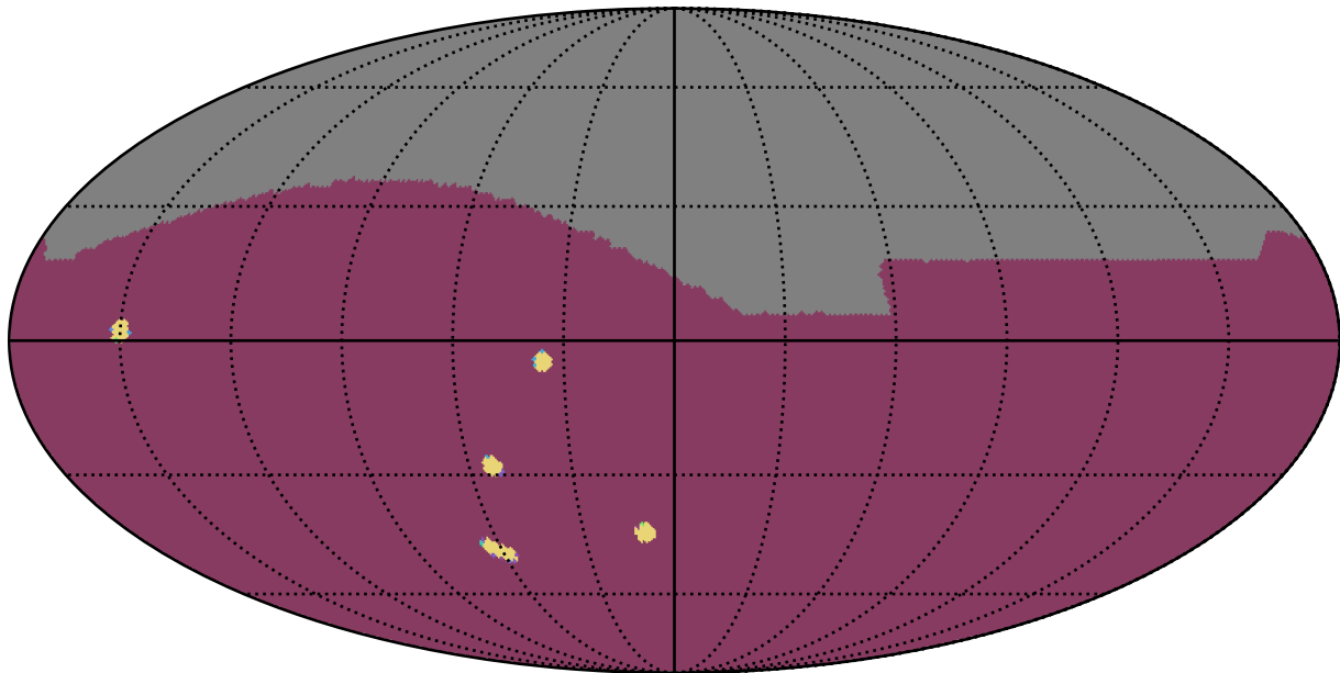
too_elab_r64_d3_ugrizy_v3.4_10yrs : NumberOfQuickRevisits
