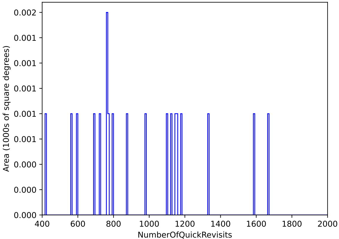
too_elab_r64_d3_ugrizy_v3.4_10yrs : NumberOfQuickRevisits
