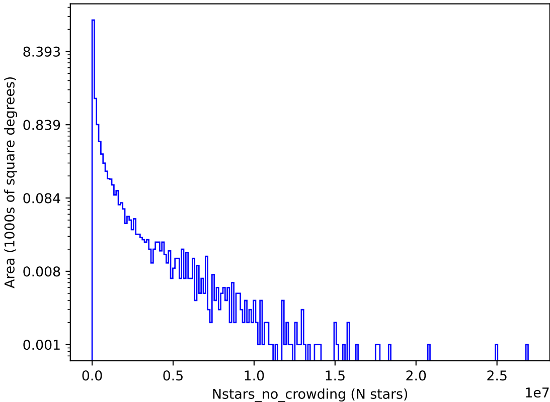
too_elab_r64_d3_ugrizy_v3.4_10yrs i: Nstars_no_crowding
