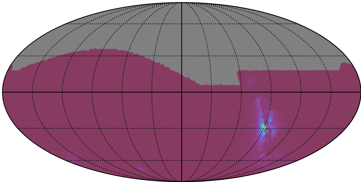
too_elab_r64_d3_ugrizy_v3.4_10yrs : NlcPoints
