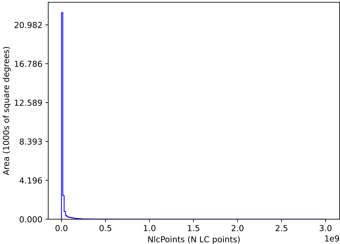
too_elab_r64_d3_ugrizy_v3.4_10yrs : NlcPoints
