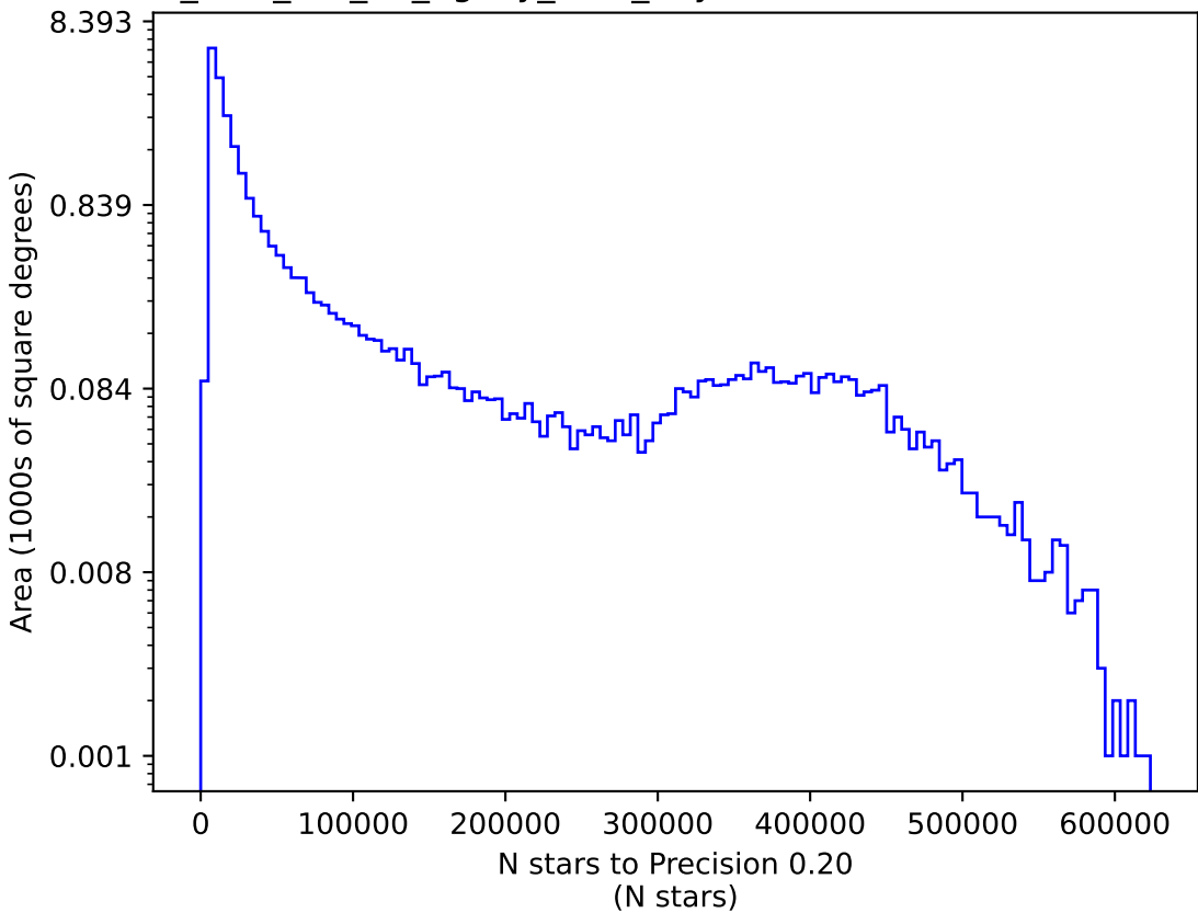
too_elab_r64_d3_ugrizy_v3.4_10yrs z: N stars to Precision 0.20
