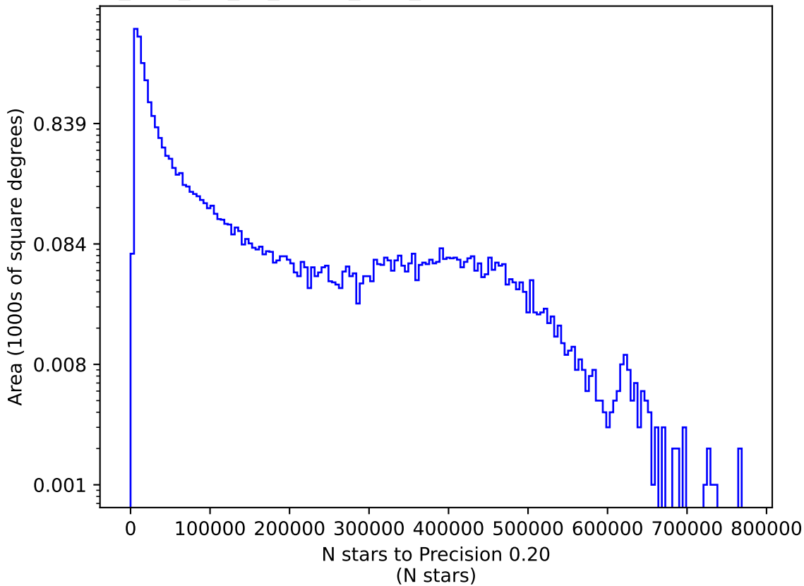
too_elab_r64_d3_ugrizy_v3.4_10yrs r: N stars to Precision 0.20
