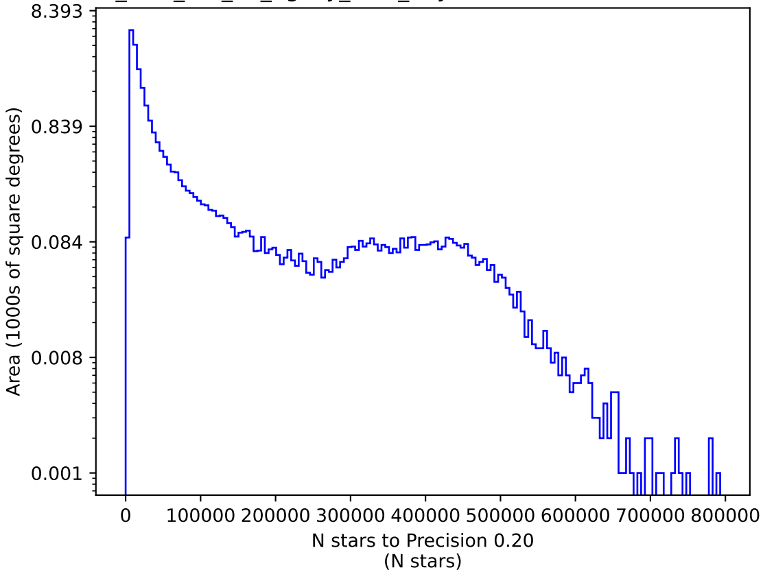
too_elab_r64_d3_ugrizy_v3.4_10yrs i: N stars to Precision 0.20
