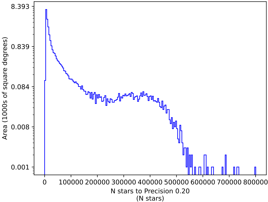
too_elab_r64_d3_ugrizy_v3.4_10yrs g: N stars to Precision 0.20
