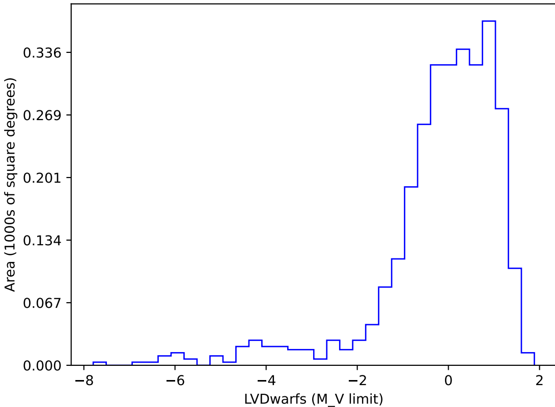
too_elab_r64_d3_ugrizy_v3.4_10yrs gi SCP: LVDwarfs
