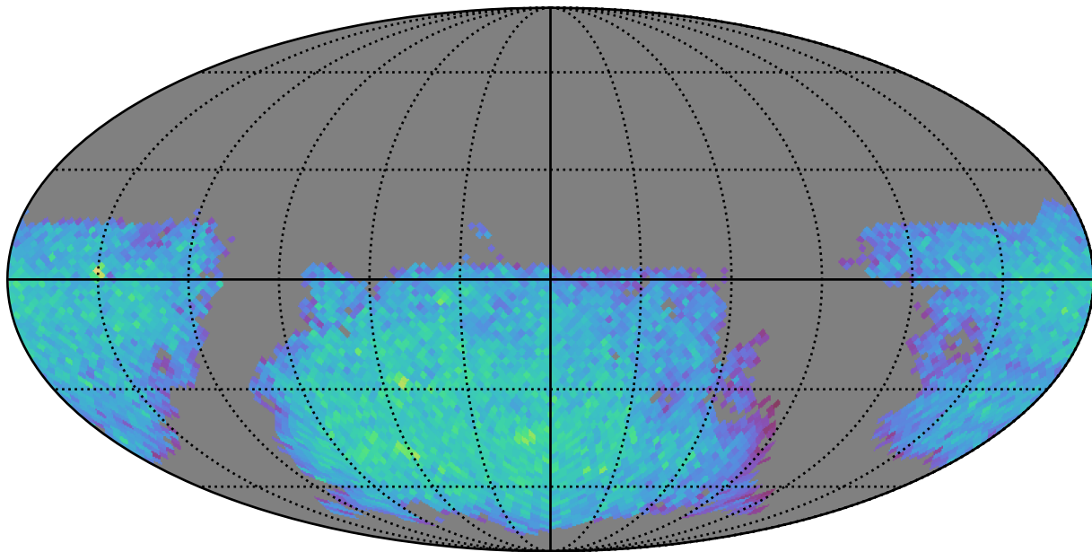
too_elab_r64_d3_ugrizy_v3.4_10yrs gi: LVDwarfs
