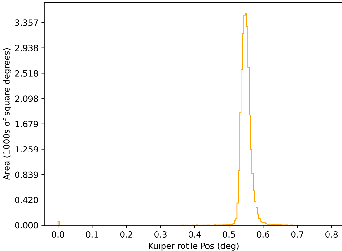
too_elab_r64_d3_ugrizy_v3.4_10yrs r: Kuiper rotTelPos
