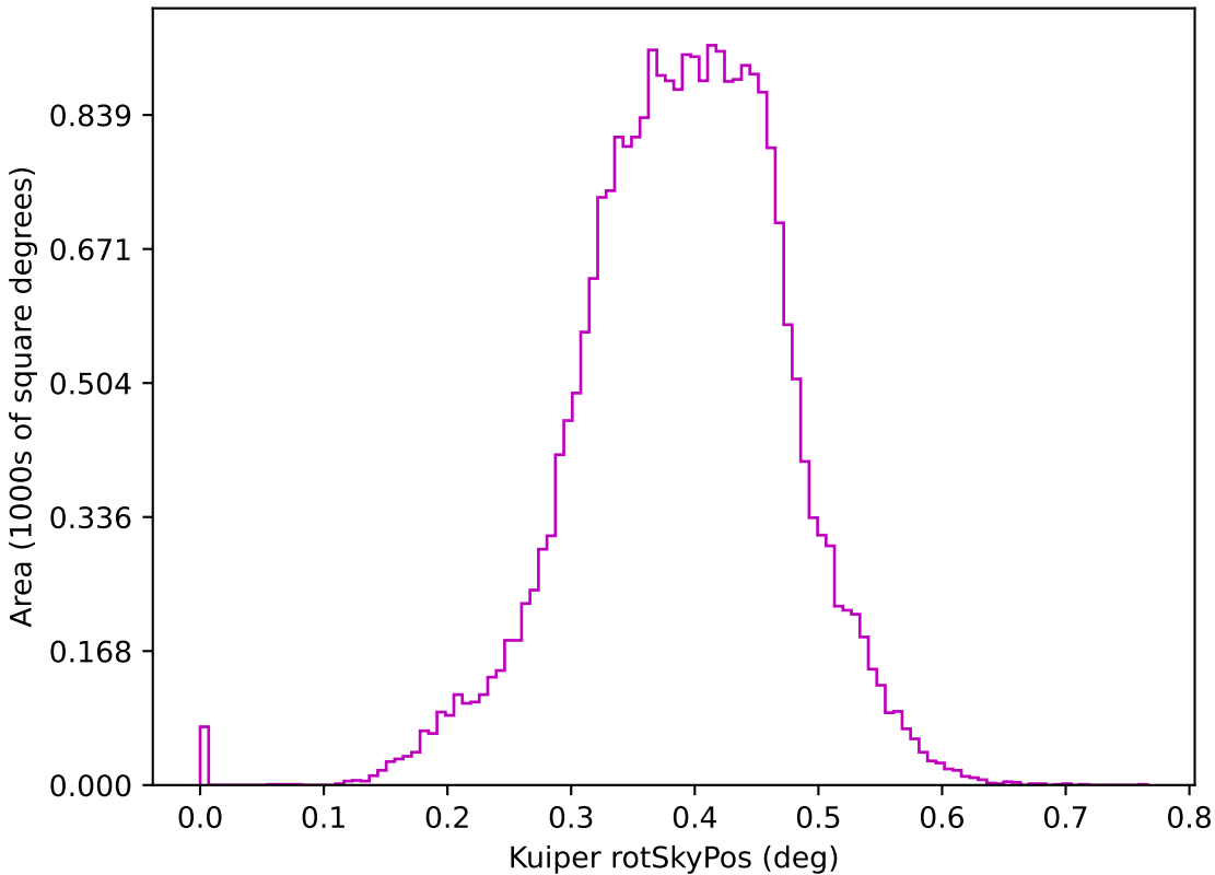
too_elab_r64_d3_ugrizy_v3.4_10yrs z: Kuiper rotSkyPos
