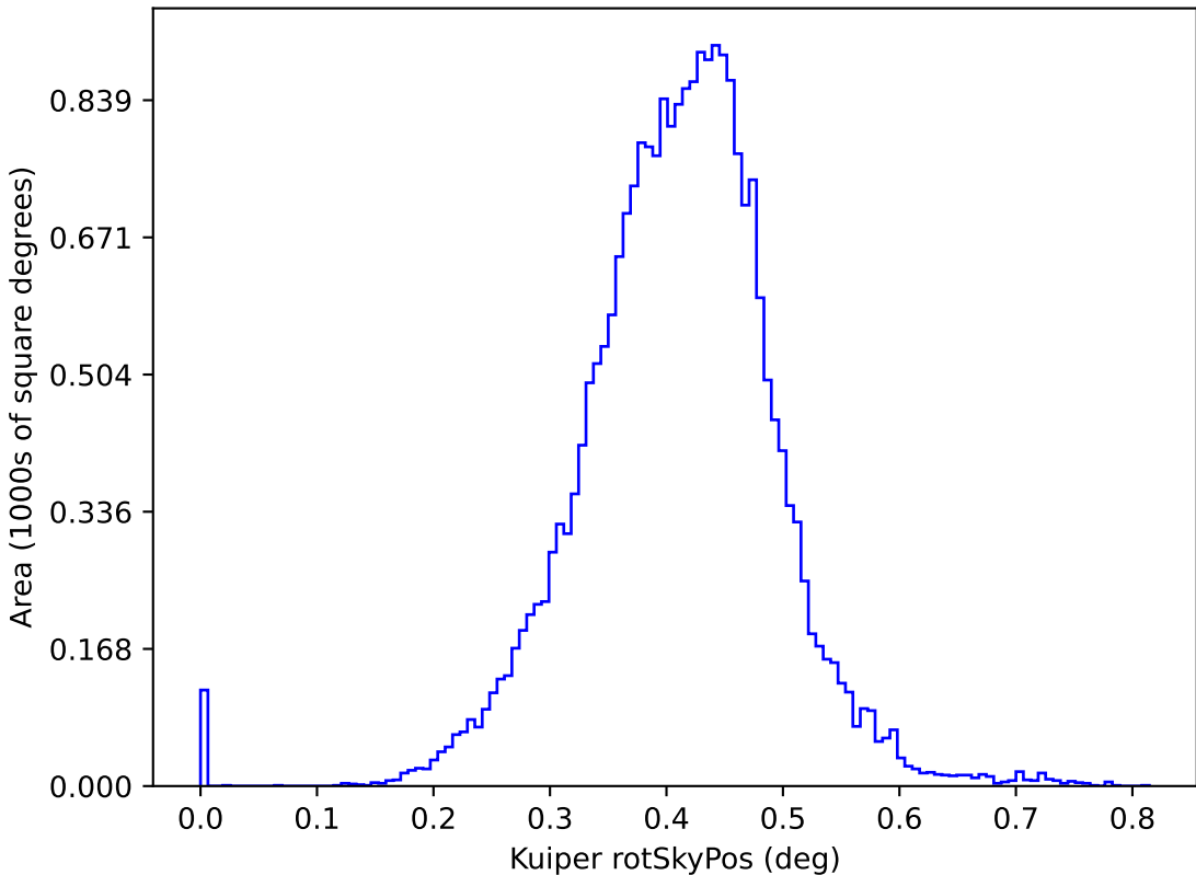
too_elab_r64_d3_ugrizy_v3.4_10yrs y: Kuiper rotSkyPos
