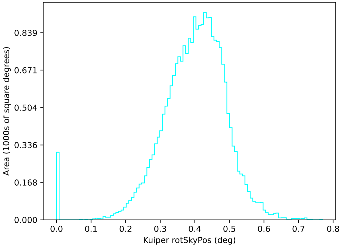
too_elab_r64_d3_ugrizy_v3.4_10yrs u: Kuiper rotSkyPos
