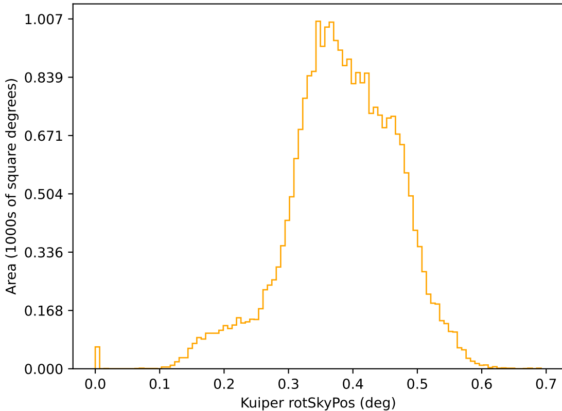
too_elab_r64_d3_ugrizy_v3.4_10yrs r: Kuiper rotSkyPos
