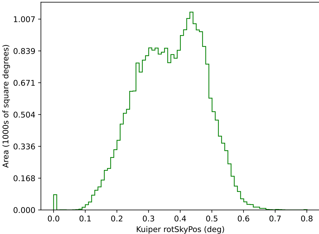
too_elab_r64_d3_ugrizy_v3.4_10yrs g: Kuiper rotSkyPos
